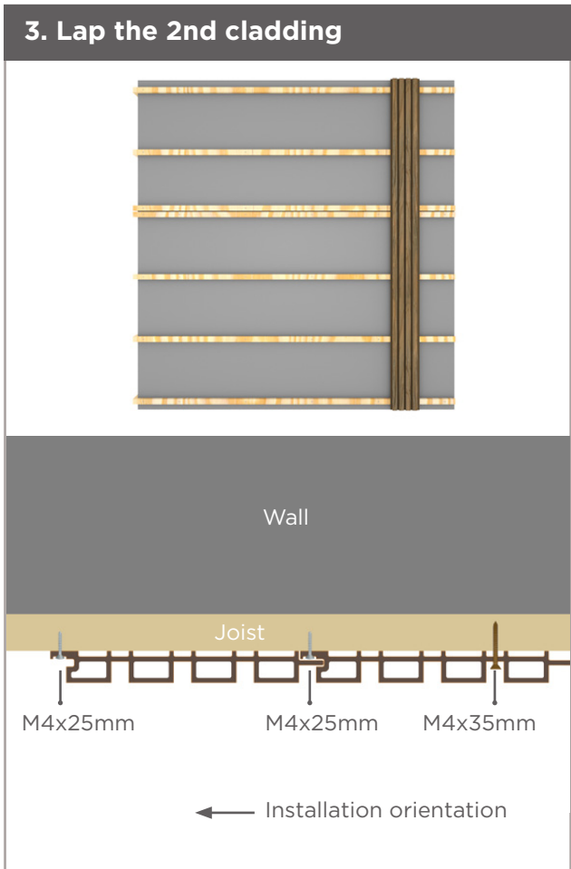
3. Lap the second cladding plank into the first. Secure the cladding to the joist using the 25mm long fixings screw through the recessed screw groove on the lap edge.
