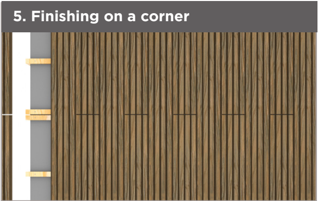
5. When finishing on a corner, cut the last cladding plank to suitable width and fix to a joist using a 35mm long colour head screw through the low valley of the cladding profile.
