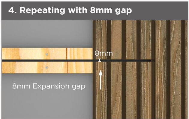
4. Continue the installation by repeating step 3. IMPORTANT: An 8mm expansion gap should be left at butt joints between two adjacent cladding planks.
